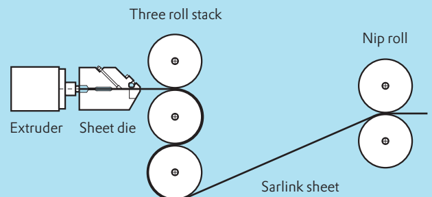
Fig. 20 - Sheet take-off
